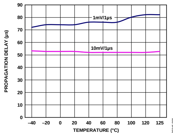
Figure 8. V_{CC} Falling Propagation Delay vs. Temperature
