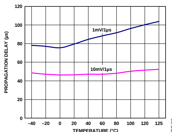
Figure 10. \text{RST IN} ( V_{TH} = 1.23\text{V} ) Falling Propagation Delay vs. Temperature
