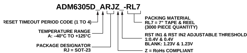
Figure 16. ADM6305 Ordering Code Structure
