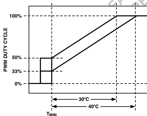
Figure 33. Adjusting \text{PWM}_{\text{MIN}} Affects T_{\text{RANGE}}
