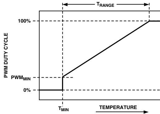
Figure 32. T_{\text{RANGE}} Parameter Affects Cooling Slope
