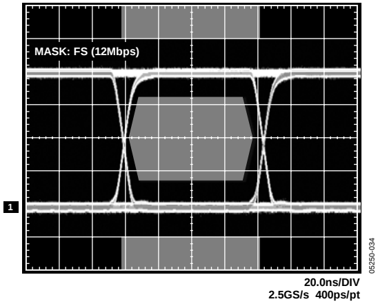
Figure 27. Eye Pattern, 12 Mbps, V_{DD} = 4.2\text{ V} , T_A = -40^\circ\text{C} , PRBS 31
