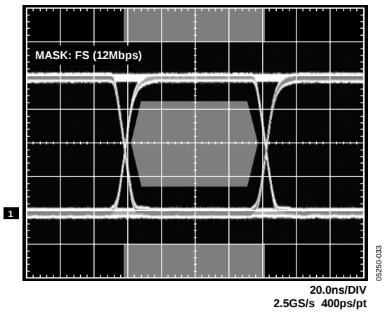
Figure 26. Eye Pattern, 12 Mbps, V_{DD} = 4.2\text{ V} , T_A = 85^\circ\text{C} , PRBS 31
