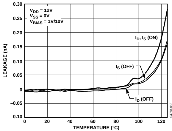
Figure 10. Leakage Currents as a Function of Temperature, Single Supply
