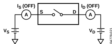
Figure 21. Off Leakage
