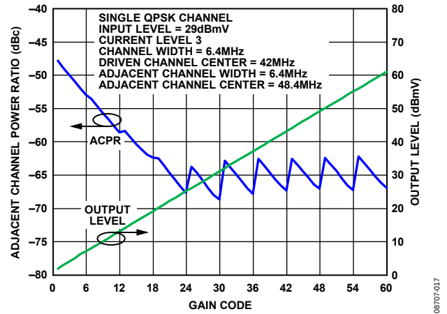
Figure 15. ACPR and Output Level vs. Gain Code
