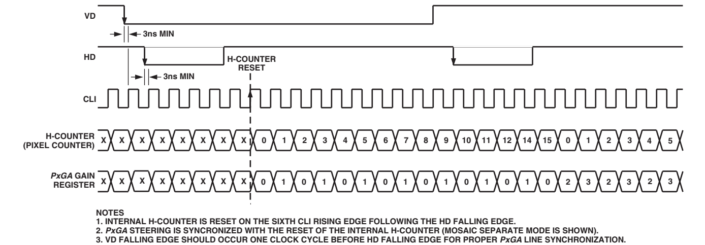
Figure 13. H-Counter Synchronization
