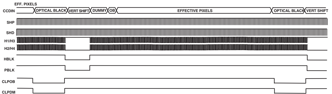
Figure 28. Sequence 3: Effective Pixels
