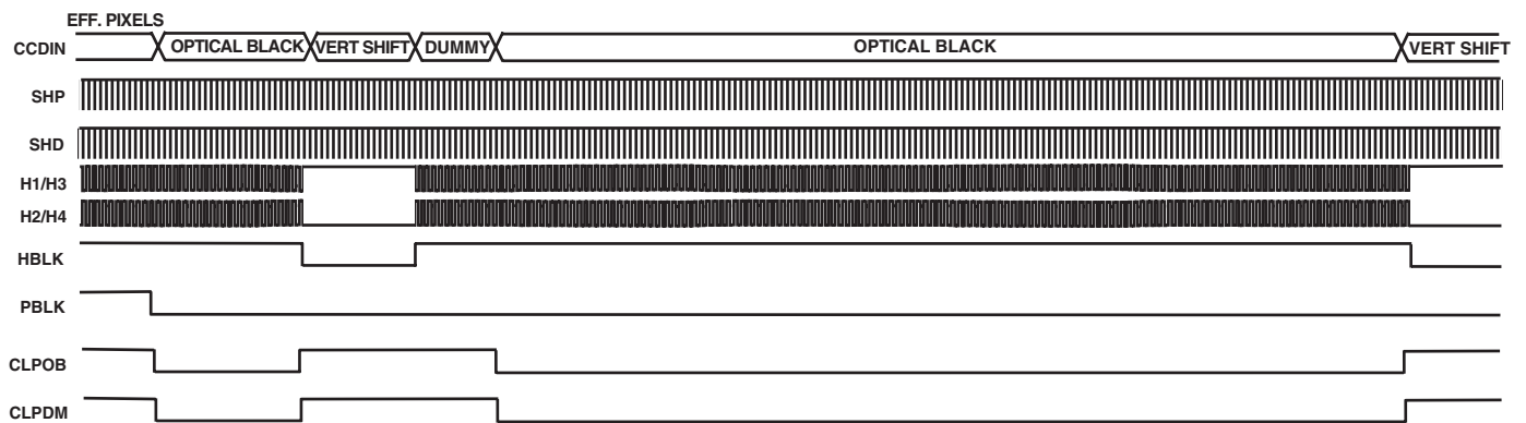
Figure 27. Sequence 2: Vertical Optical Black
