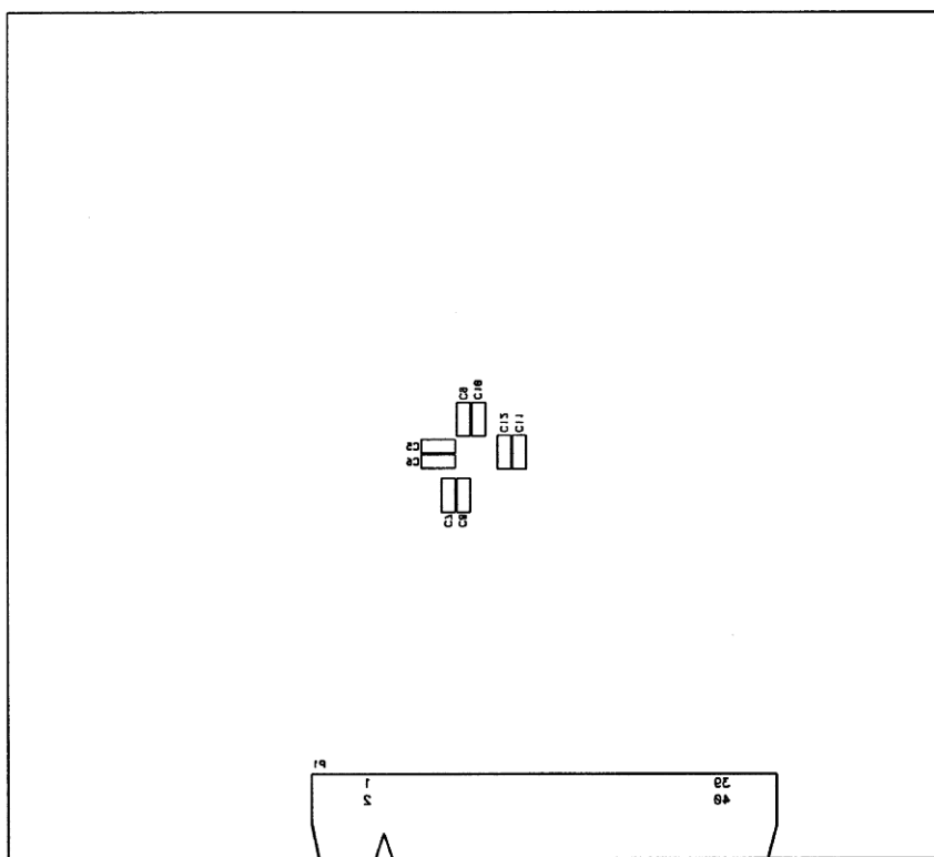
Figure 67. Silkscreen Layer—Bottom
