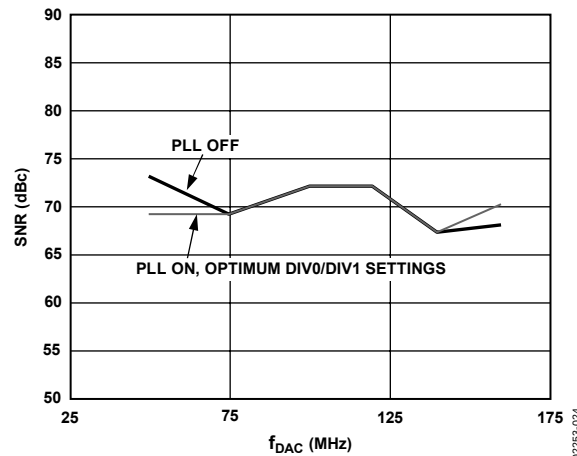
Figure 24. SNR vs. f_{DATA} @ f_{OUT} = 10 MHz
