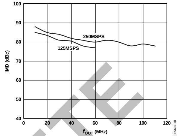
Figure 10. AD9741 IMD vs. f_{OUT} , Normal Mode
