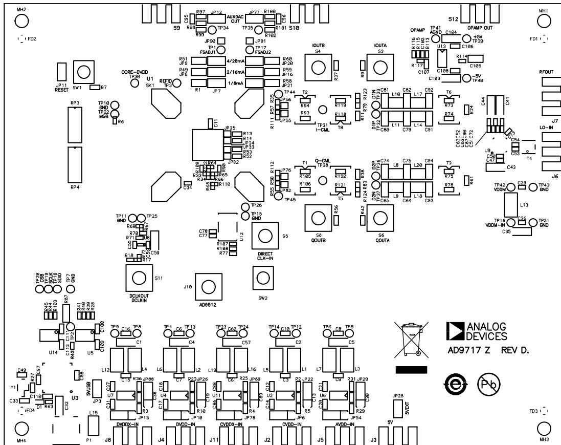
Figure 129. Silkscreen—Primary Side
