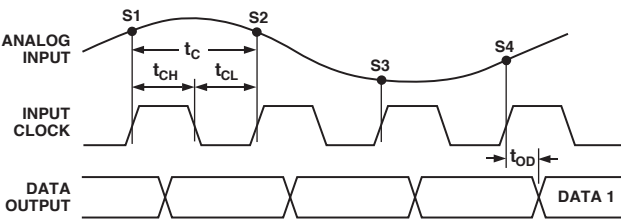
Figure 1. Timing Diagram
