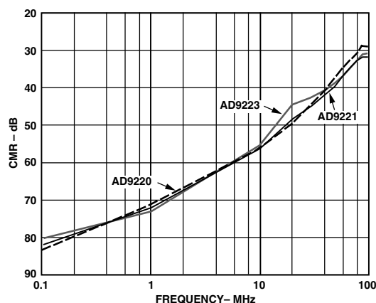
Figure 11. AD9221/AD9223/AD9220 Input CMR vs. Input Frequency
