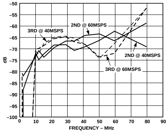
TPC 3. Harmonics vs. AIN Frequency
