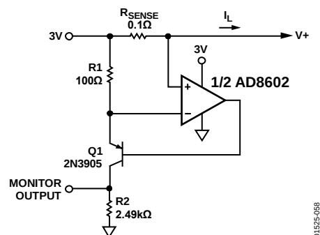
Figure 58. High-Side Current Monitor
