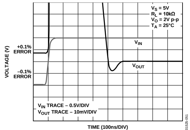
Figure 51. Settling Time
