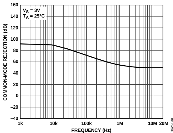
Figure 30. Common-Mode Rejection Ratio vs. Frequency
