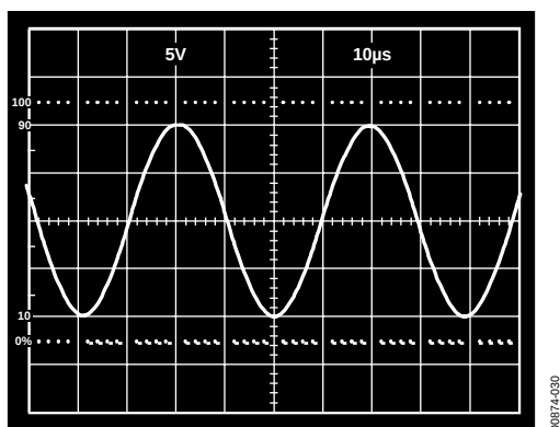
Figure 30. 20 V p-p, 25 kHz Sine Wave Input; Unity-Gain Follower; V_S = \pm 15\text{ V} , R_L = 600\ \Omega
