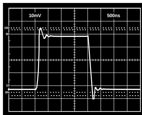
Figure 33. Small Signal Response Unity-Gain Follower; V_S = \pm 15\text{ V} , R_L = 10\text{ k}\Omega
