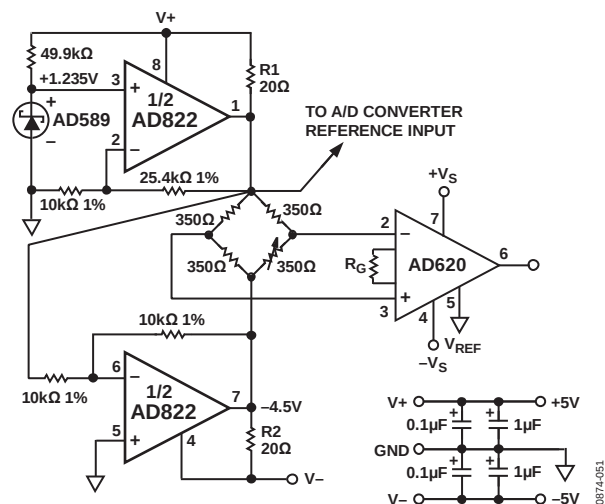
Figure 50. Low Dropout Bipolar Bridge Driver
