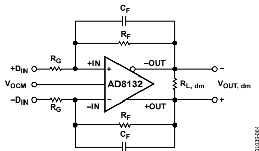
Figure 64. Circuit Definitions
