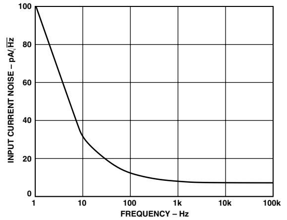
TPC 15. Noise vs. Frequency; V_S = \pm 5V
