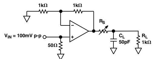
Figure 7. Capacitive Load Drive Circuit
