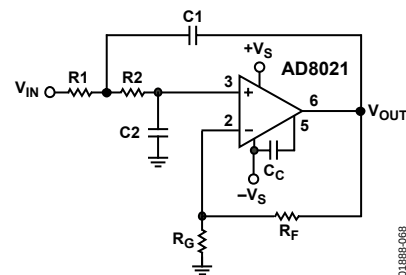
Figure 68. Schematic of a Second-Order, Low-Pass Active Filter
