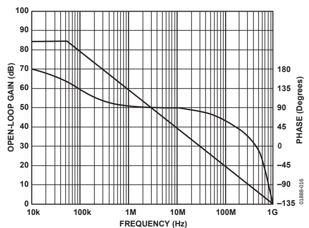
Figure 16. Open-Loop Gain and Phase vs. Frequency, R_G = 100 Ω, R_F = 1 kΩ, R_O = 976 Ω, R_D = 53.6 Ω, C_C = 0 pF (See Figure 50)
