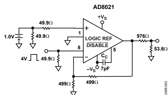
Figure 53. Enable/Disable
