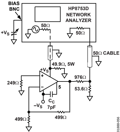
Figure 56. Positive PSRR
