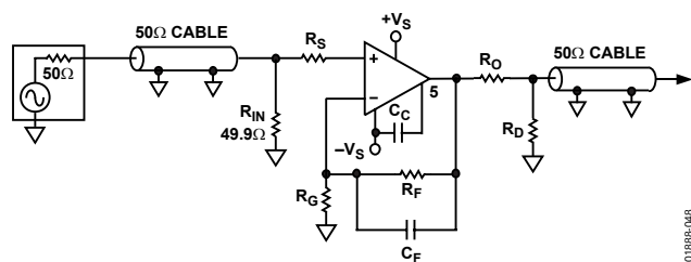
Figure 48. Noninverting Gain
