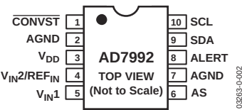
Figure 3. AD7992 Pin Configuration
