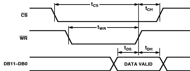
Figure 3. AD7945 Timing Diagram
