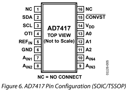
Figure 6. AD7417 Pin Configuration (SOIC/TSSOP)
