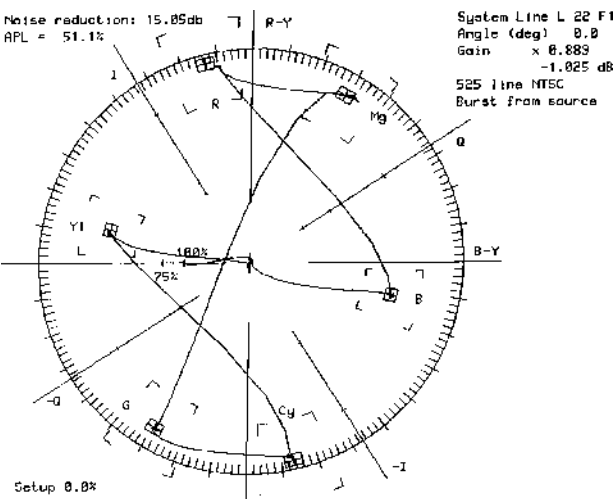
Figure 6. 100% Color Bars on Vector Scope, NTSC
