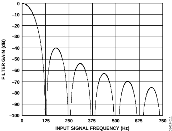
Figure 12. Filter Response
