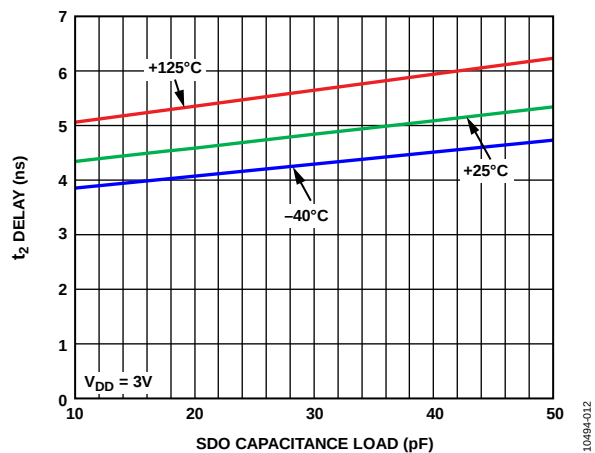
Figure 12. t_2 Delay vs. SDO Capacitance Load, V_{DD} = 3\text{V}
