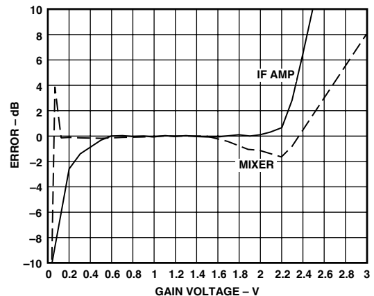
TPC 8. Gain Error vs. Gain Control Voltage, Representative Part
