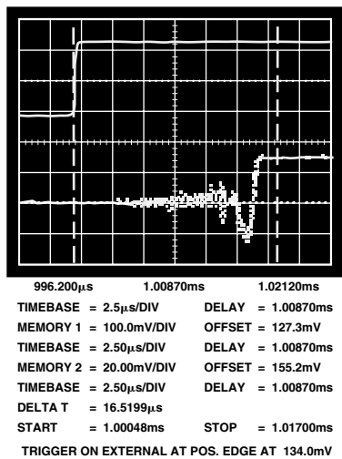
TPC 9. PLL Acquisition Time
