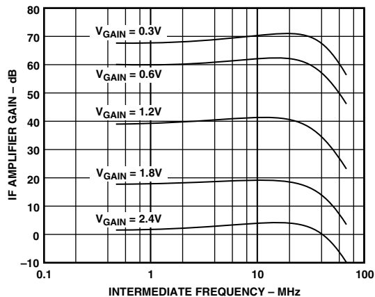
TPC 7. IF Amplifier Gain vs. Frequency, T = 25^{\circ}C , V_{POS} = 3V , V_{REF} = 1.5V
