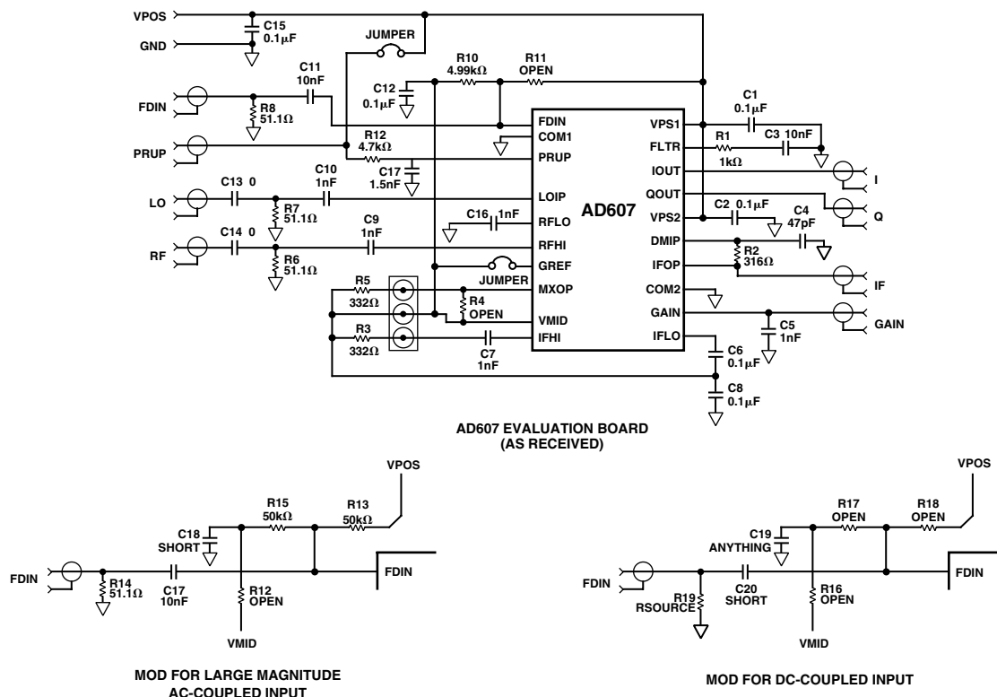
Figure 26. Evaluation Board
