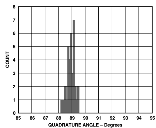
TPC 12. Demodulator Quadrature Angle, Histogram, T = 25^{\circ}C , V_{POS} = 3V , IF = 10.7MHz
