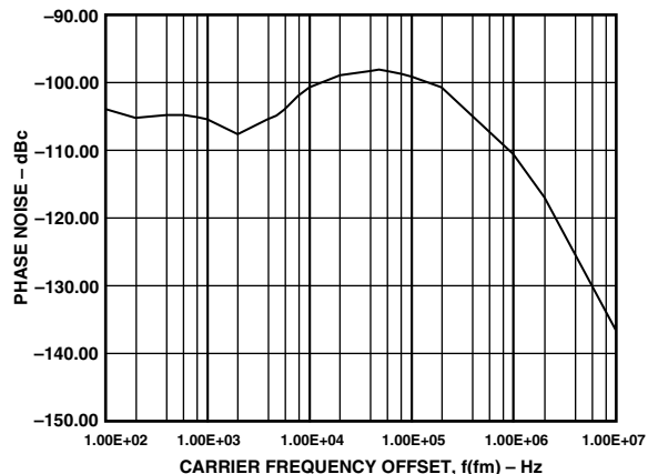
TPC 10. PLL Phase Noise L(F) vs. Frequency, V_{POS} = 3V , C3 = 0.1\mu F , IF = 10.7MHz
