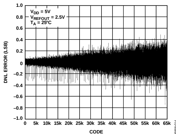
Figure 13. DNL—AD5663R-5
