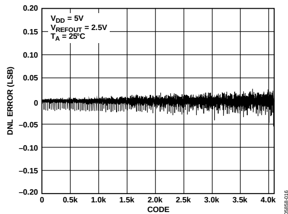
Figure 15. DNL—AD5623R-5
