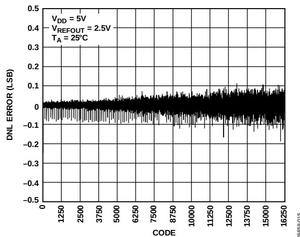
Figure 14. DNL—AD5643R-5
