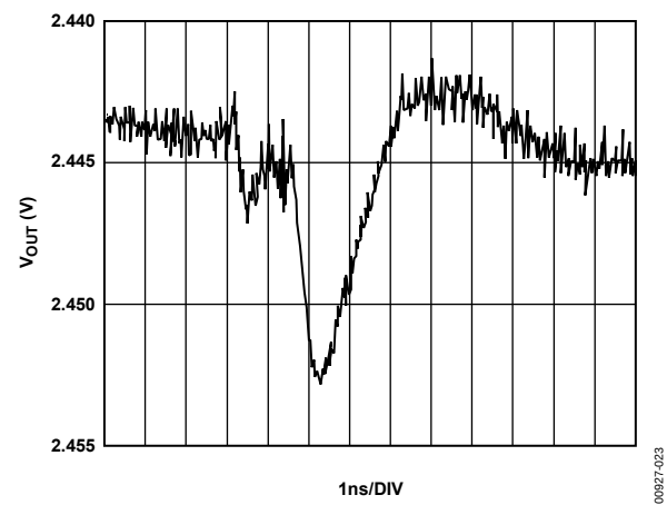
Figure 23. Digital Feedthrough
