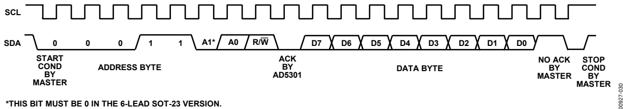
Figure 32. AD5301 Readback Sequence
