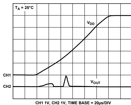
Figure 20. Power-On Reset to 0 V
