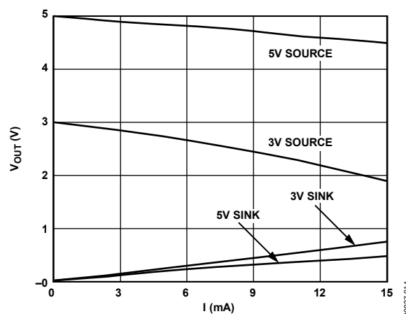
Figure 14. Source and Sink Current Capability
