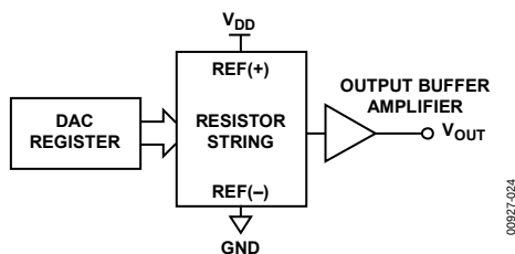
Figure 24. DAC Channel Architecture
