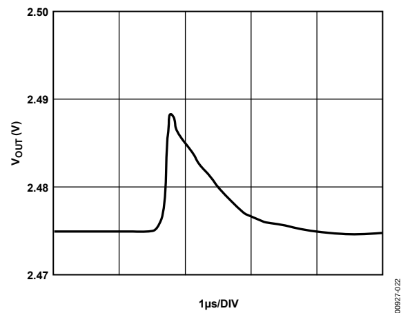
Figure 22. Major-Code Transition
