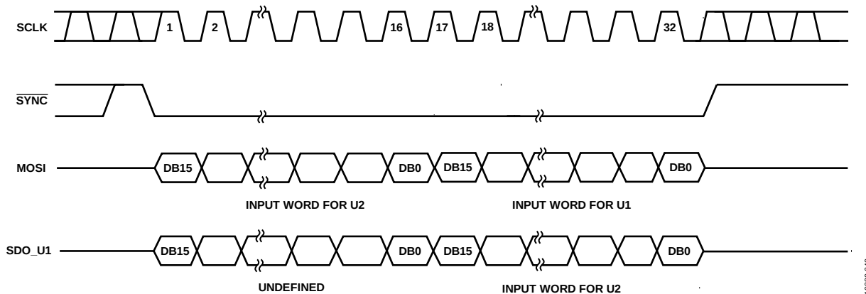
Figure 41. Daisy-Chain Diagram
