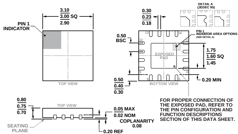
Figure 47. 16-Lead Lead Frame Chip Scale Package [LFCSP] 3 mm x 3 mm Body and 0.75 mm Package Height (CP-16-22)
