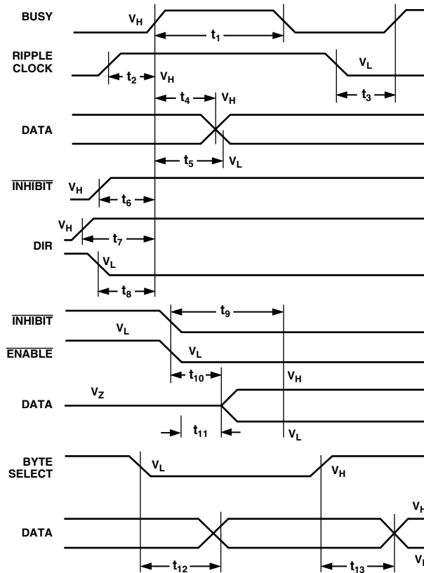
Figure 3. Digital Timing
