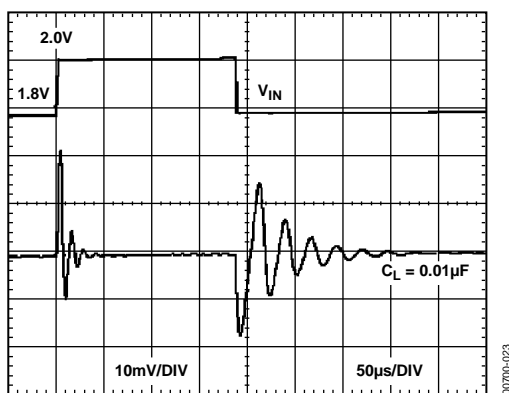
Figure 23. Transient Response with Capacitive Load
