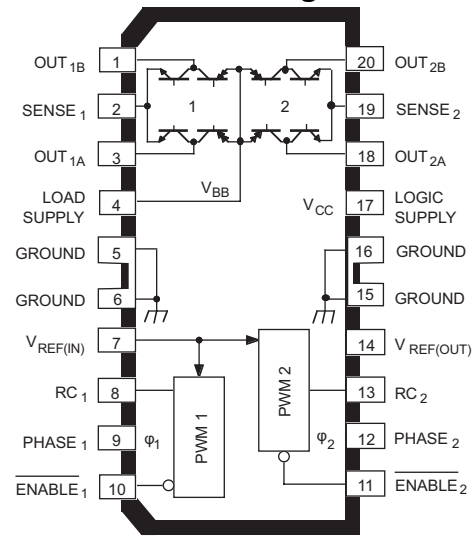
Pin-out Diagram
