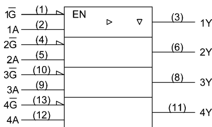
74HC125D
