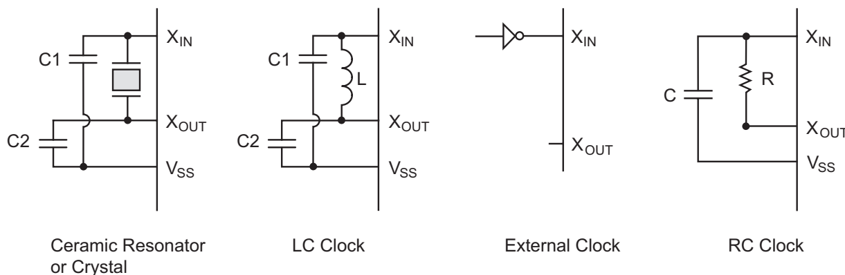
Figure 18. Oscillator Configuration
