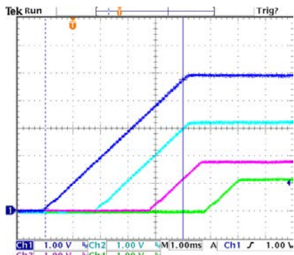
Fig. 14: Sequential Start-up CH1:3.3V, CH2:5V, CH3:1V, CH4:1.8V
