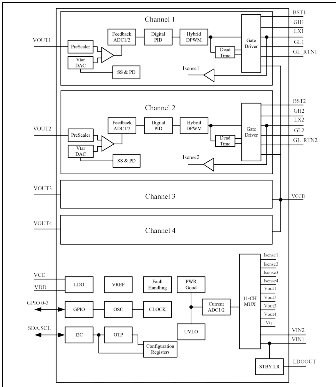
Fig. 2: XRP7714 Block Diagram
