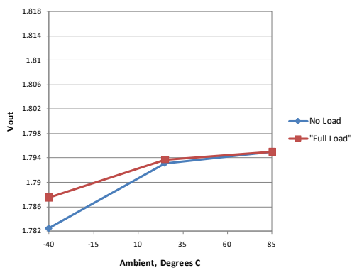
Fig. 18: Temperature Regulation 1.8V out ( \pm 1\% Vout window)
