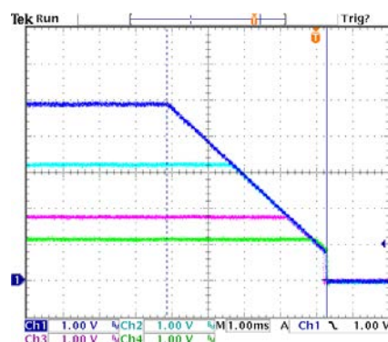
Fig. 15: Sequential Soft-stop V OUT Shutdown=0.8V, 3A load CH1:3.3V, CH2:5V, CH3:1V, CH4:1.8V
