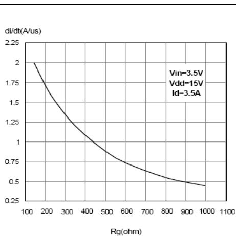
Figure 28. Turn-on current slope ( V_{in}=3.5V )
