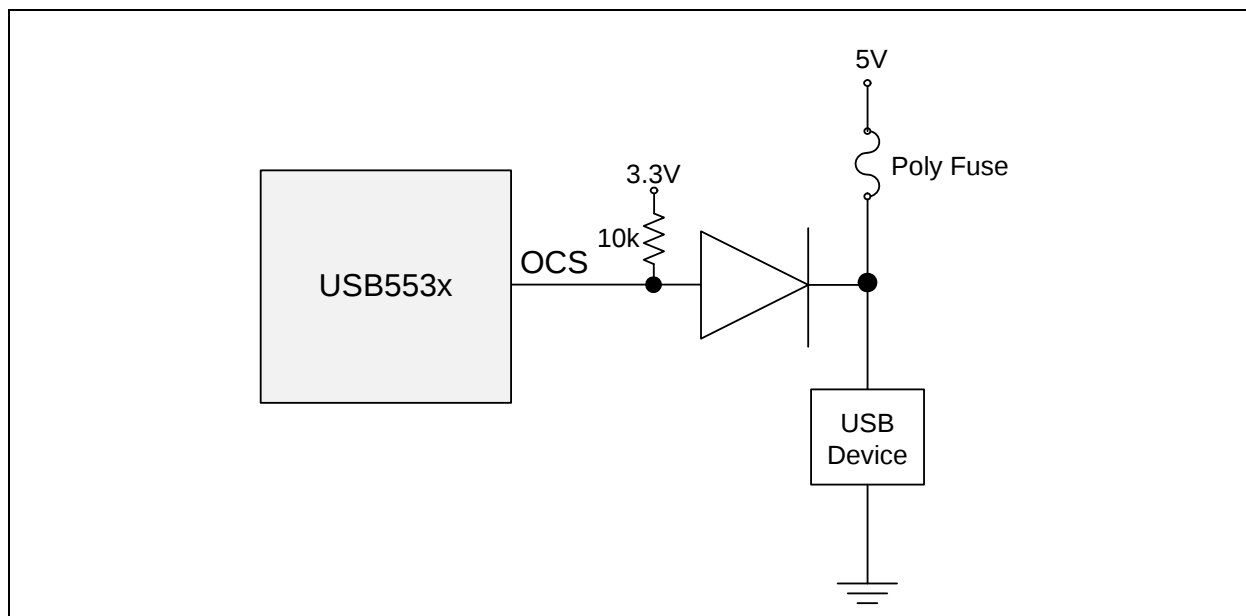
FIGURE 4-13: POLY-FUSE IMPLEMENTATION
