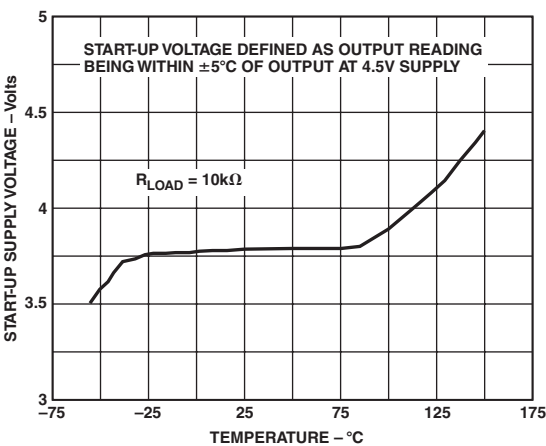
TPC 16. Start-Up Voltage vs. Temperature
