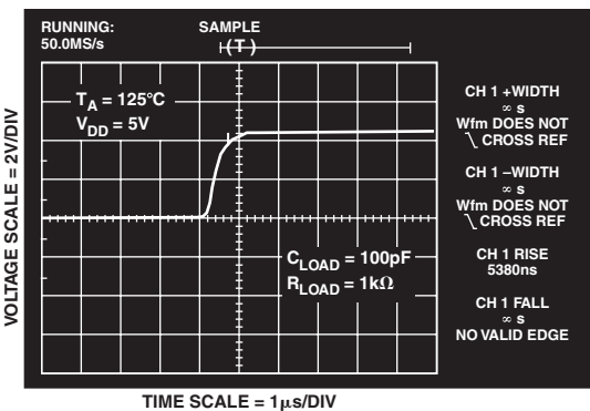
TPC 6. TMP03 Output Rise Time at 125°C
