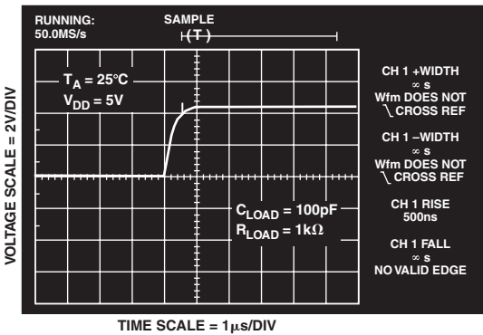
TPC 5. TMP03 Output Rise Time at 25°C
