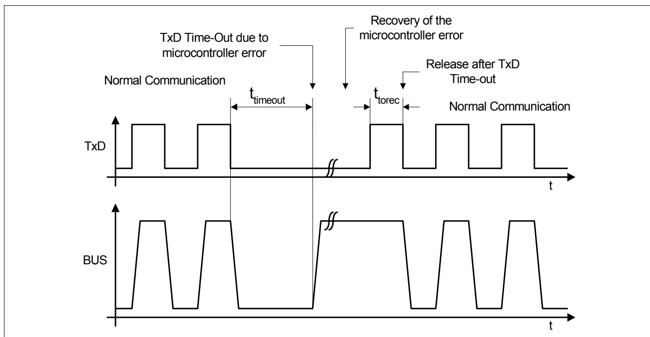
Figure 10 TxD Time-Out function
