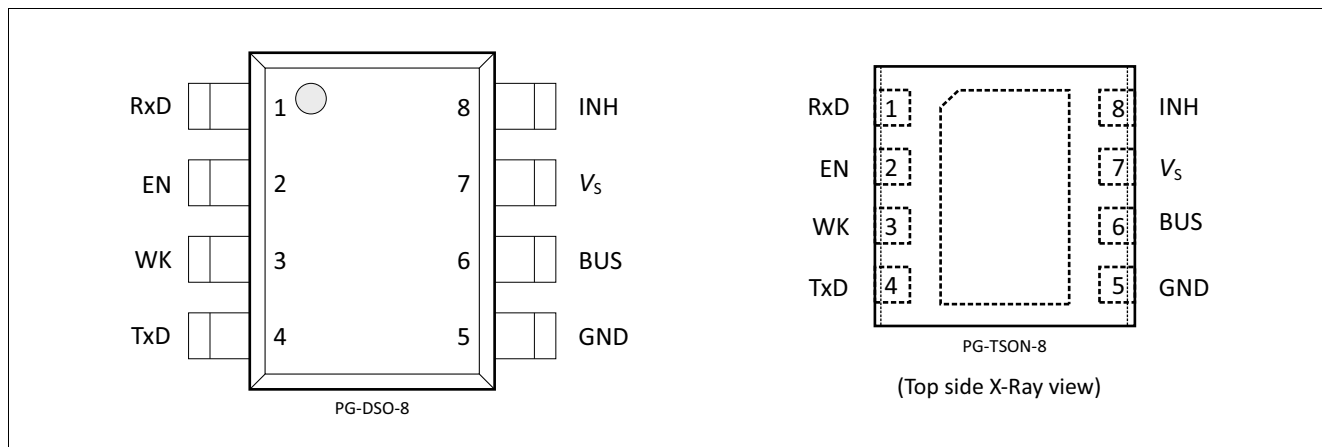
Figure 2 Pin Configuration
