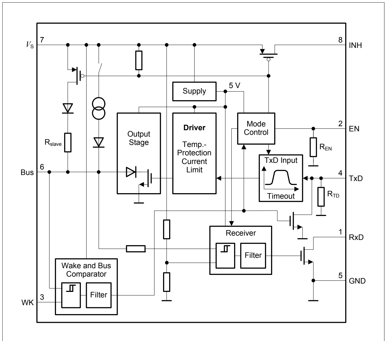
Figure 1 Block Diagram
