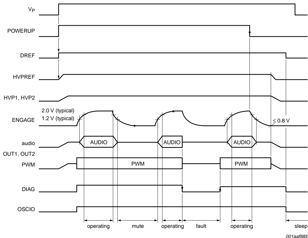
Fig 4. Start-up sequence
