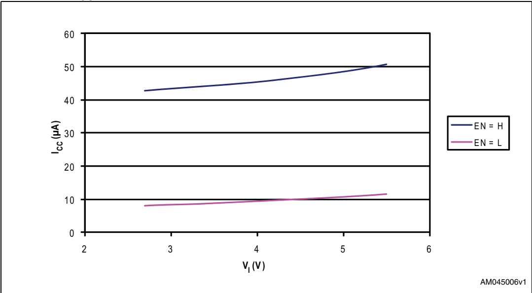
Figure 19. I_{CC} versus V_I
