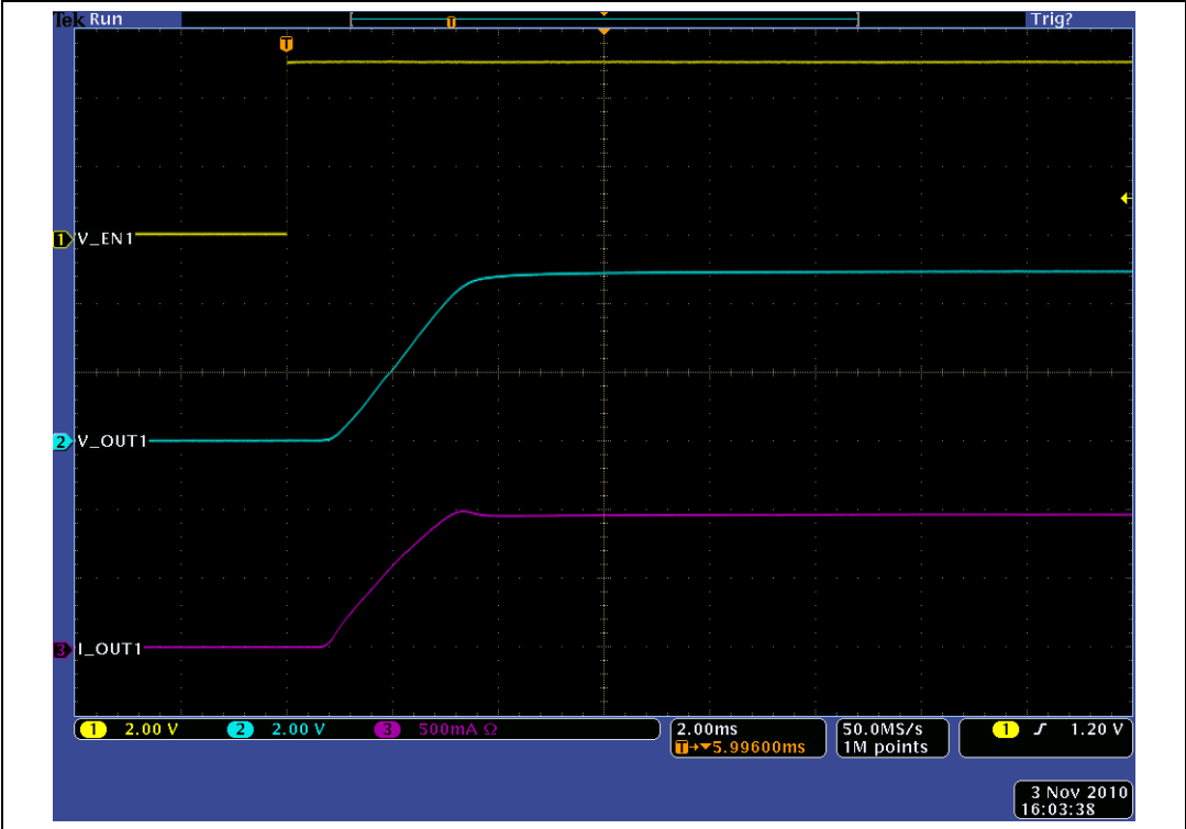
Figure 30. Turn-on for C_{LOAD} = 100\ \mu F
