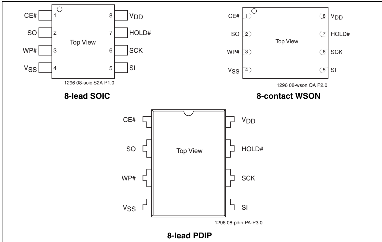
FIGURE 2-1: PIN ASSIGNMENTS
