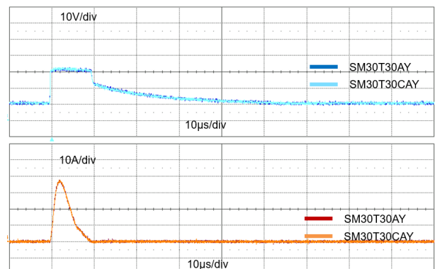
Figure 14. ISO7637-2 pulse 2a response ( V_S = 112\text{ V} ) with 12 V battery
