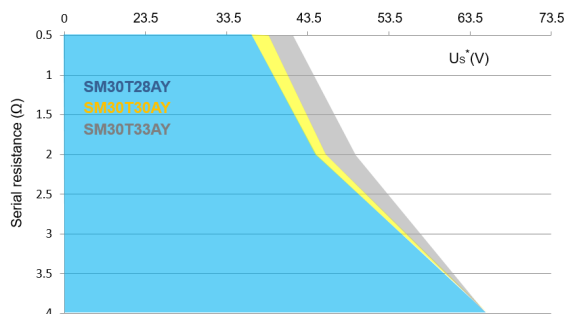
Figure 21. Load dump capability (typical values, U_s^* = f(R_i) test B, U_s = 87\text{ V} , t_p = 150\text{ ms} )
