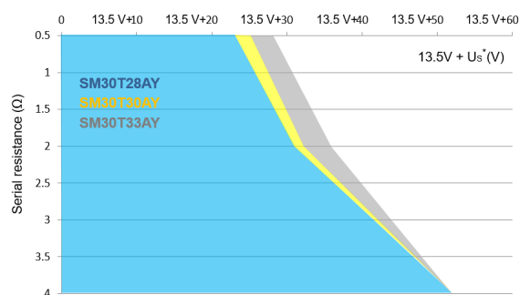
Figure 18. Load dump capability (typical values, U_s^* = f(R_i) pulse 5b, U_s = 87\text{ V} , t_p = 150\text{ ms} )
