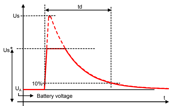
Figure 20. ISO16750-2 test B definition
