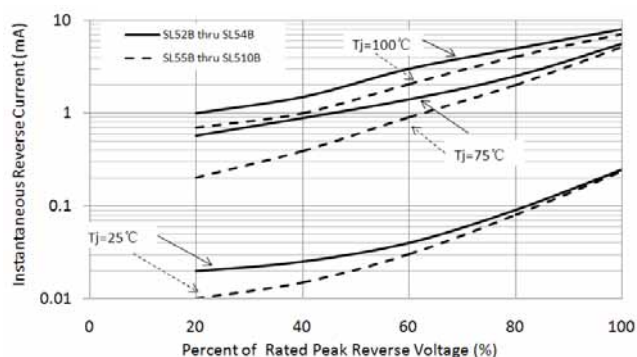
Figure 4. Typical Reverse Characteristics
