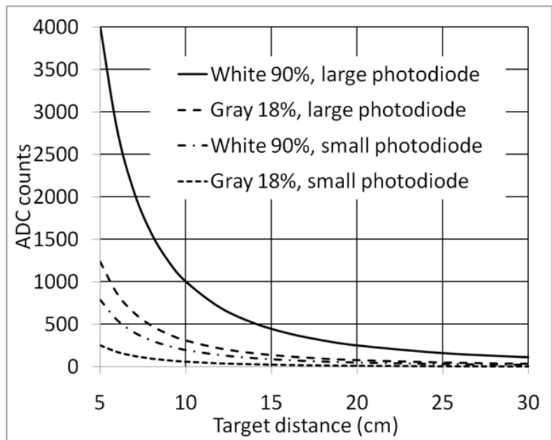
Figure 3. Proximity response using Kodak gray cards, PS_RANGE=0, PS_ADC_GAIN=0 (single 25.6 \mu s LED pulse), \pm 22^\circ LED view angle, 850 nm, 22.5 mW/sr, no overlay, 5 mm LED center to Si114x center
