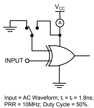
Figure 3. I_{cCD} Test Circuit
