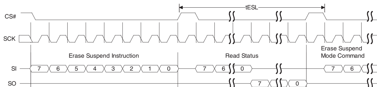
Figure 111. Erase Suspend Command Sequence
