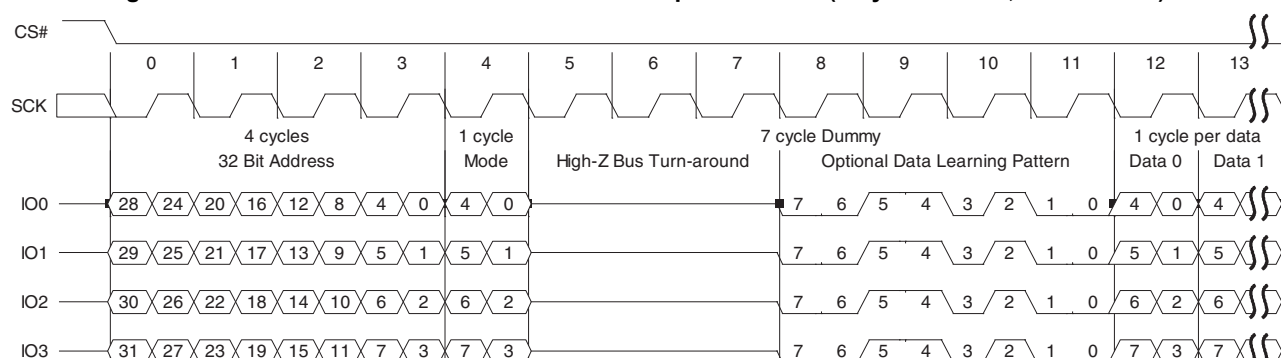
Figure 97. Continuous DDR Quad I/O Read Subsequent Access (4-byte Address, EHPLC=01b) [46]
