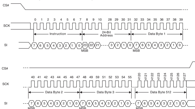
Figure 113. OTP Program Command Sequence
