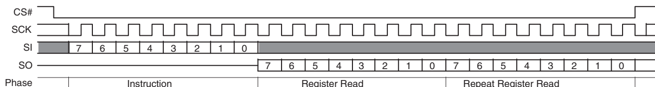
Figure 122. PPB Lock Register Read Command Sequence
