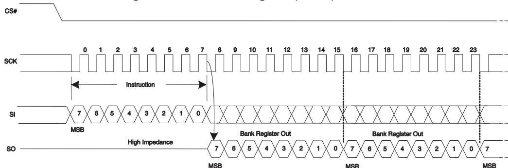
Figure 51. Read Bank Register (BRRD) Command
