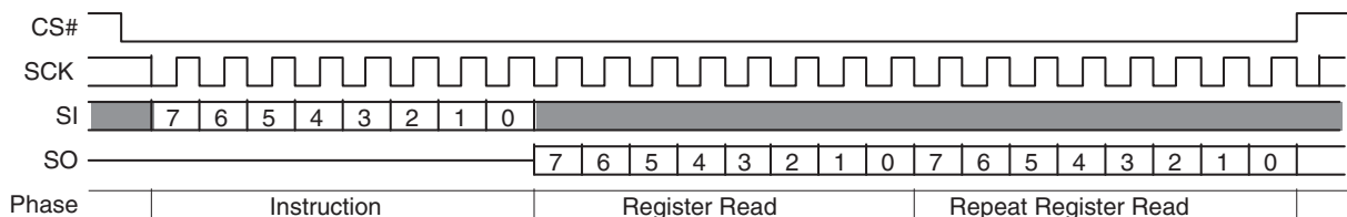
Figure 50. Read Configuration Register (RDCR) Command Sequence
