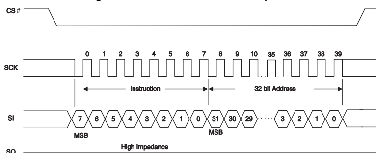
Figure 120. PPBP Command Sequence
