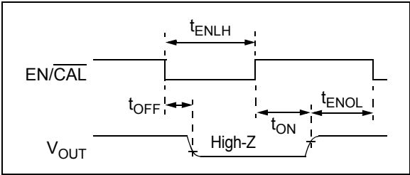
FIGURE 1-5: EN/CAL Timing Diagram.
