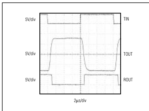
Figure 7. Loopback Test Result at 120kbps
