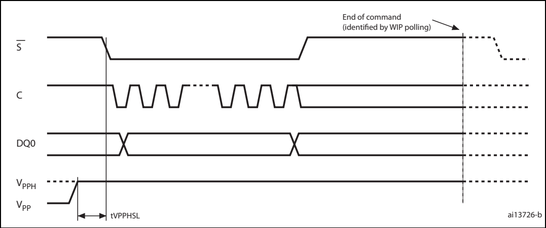
Figure 35. V_{PPH} timing
