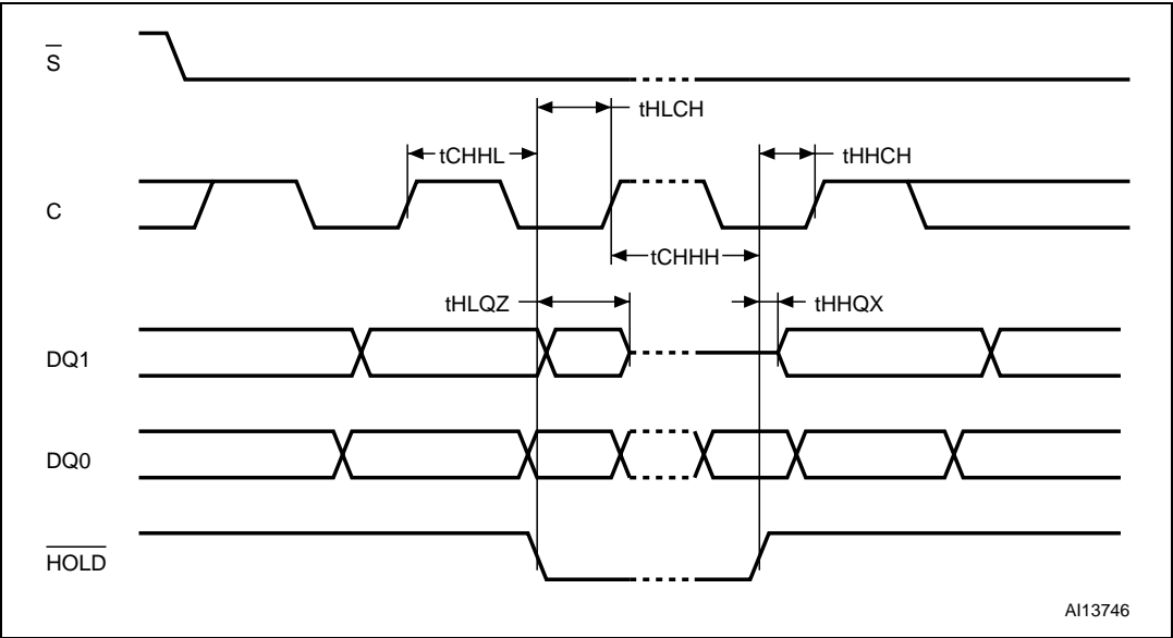
Figure 33. Hold timing
