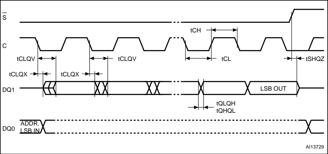
Figure 34. Output timing
