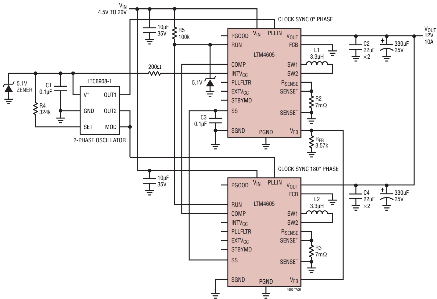
Figure 18. Two-Phase Parallel, 12V at 10A Design
