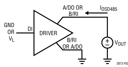
Figure 2. RS485 Driver Output Current
