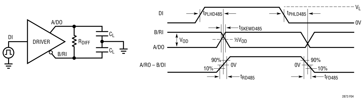
Figure 4. RS485 Driver Timing Measurement
